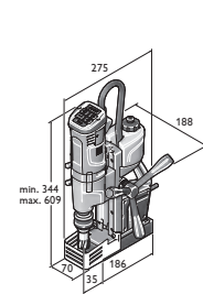
KBU 35-2 Q KBU 35-2 QW
